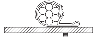
UGCTE Bundle is offset from mounting point
