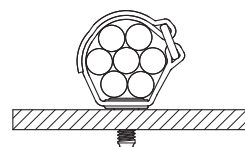
UGCTC Bundle is centered over mounting point
